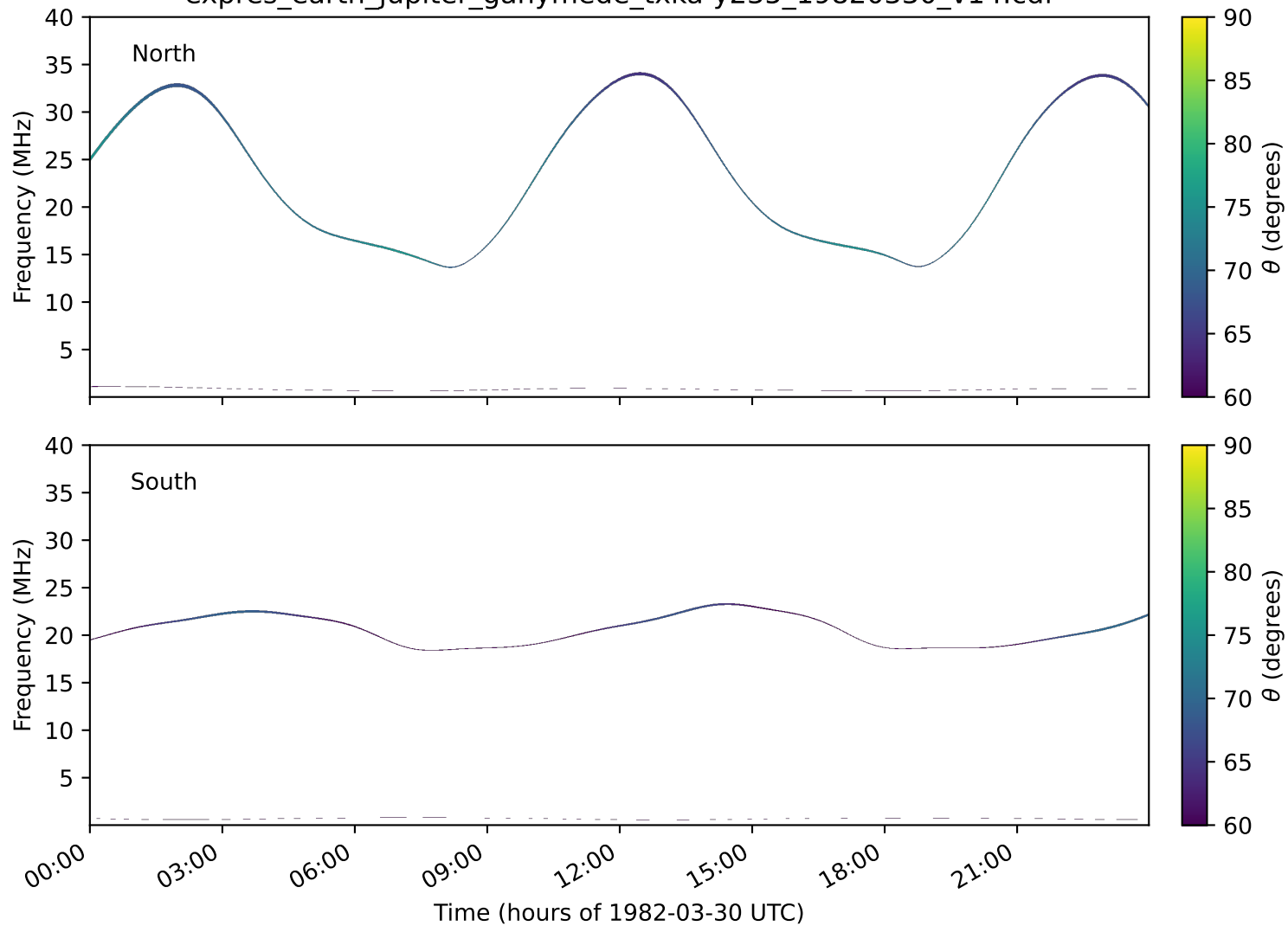
expres_earth_jupiter_ganymede_txka-y235_19820330_v14.cdf
