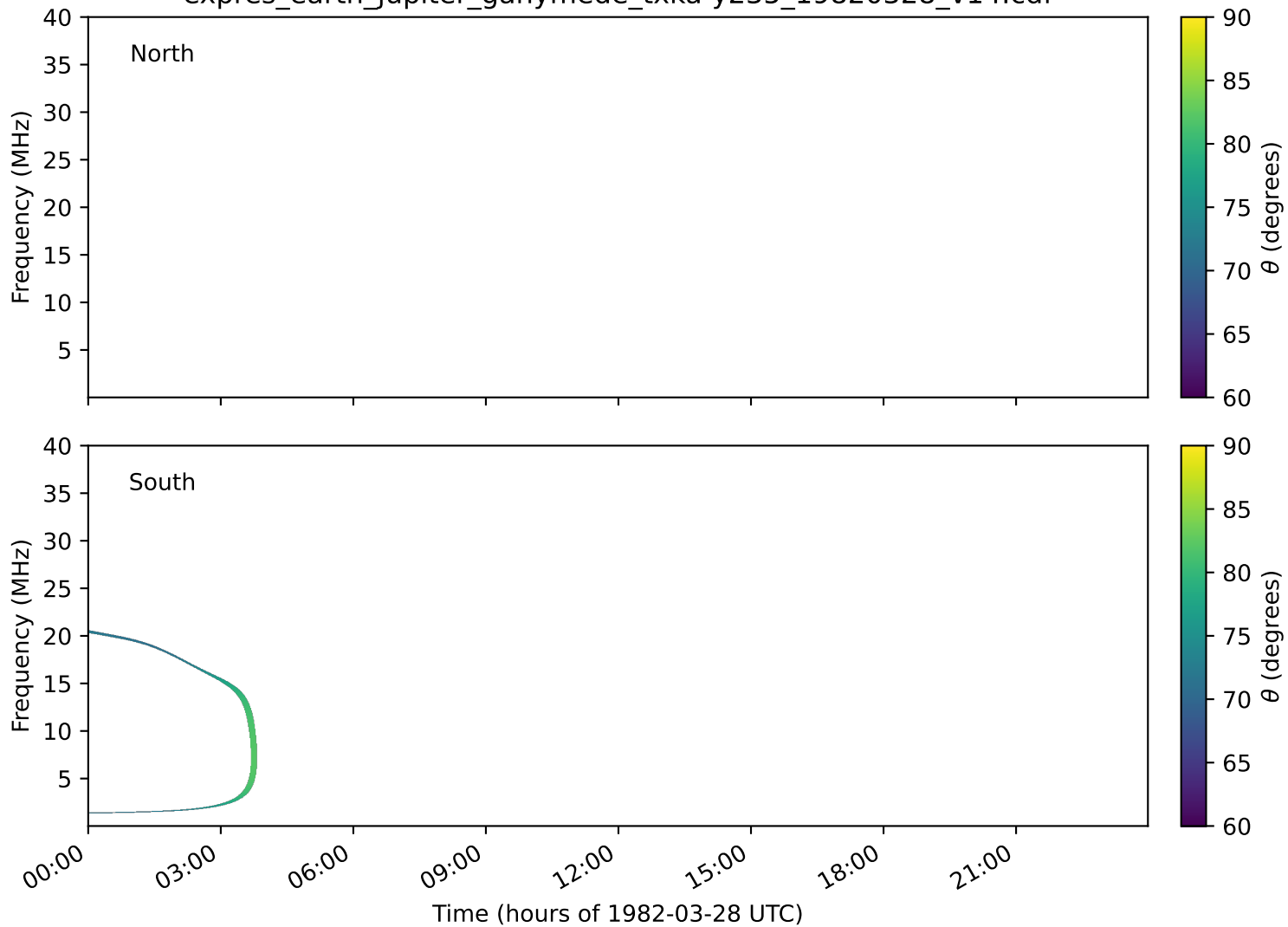
expres_earth_jupiter_ganymede_txka-y235_19820328_v14.cdf
