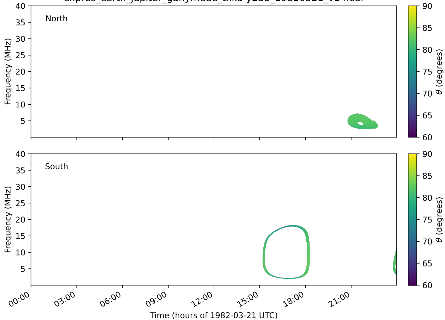
expres_earth_jupiter_ganymede_txka-y235_19820321_v14.cdf
