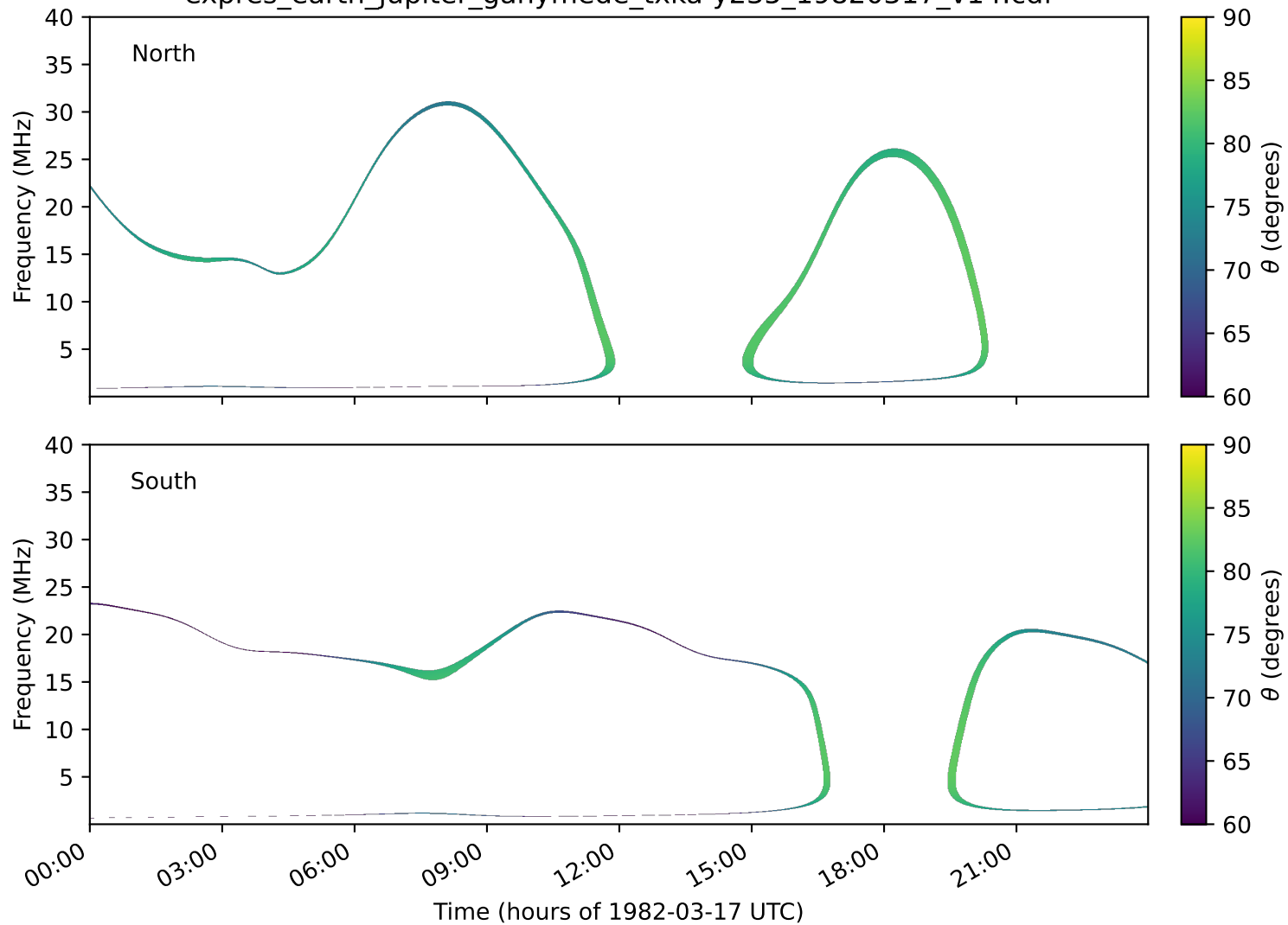
expres_earth_jupiter_ganymede_txka-y235_19820317_v14.cdf
