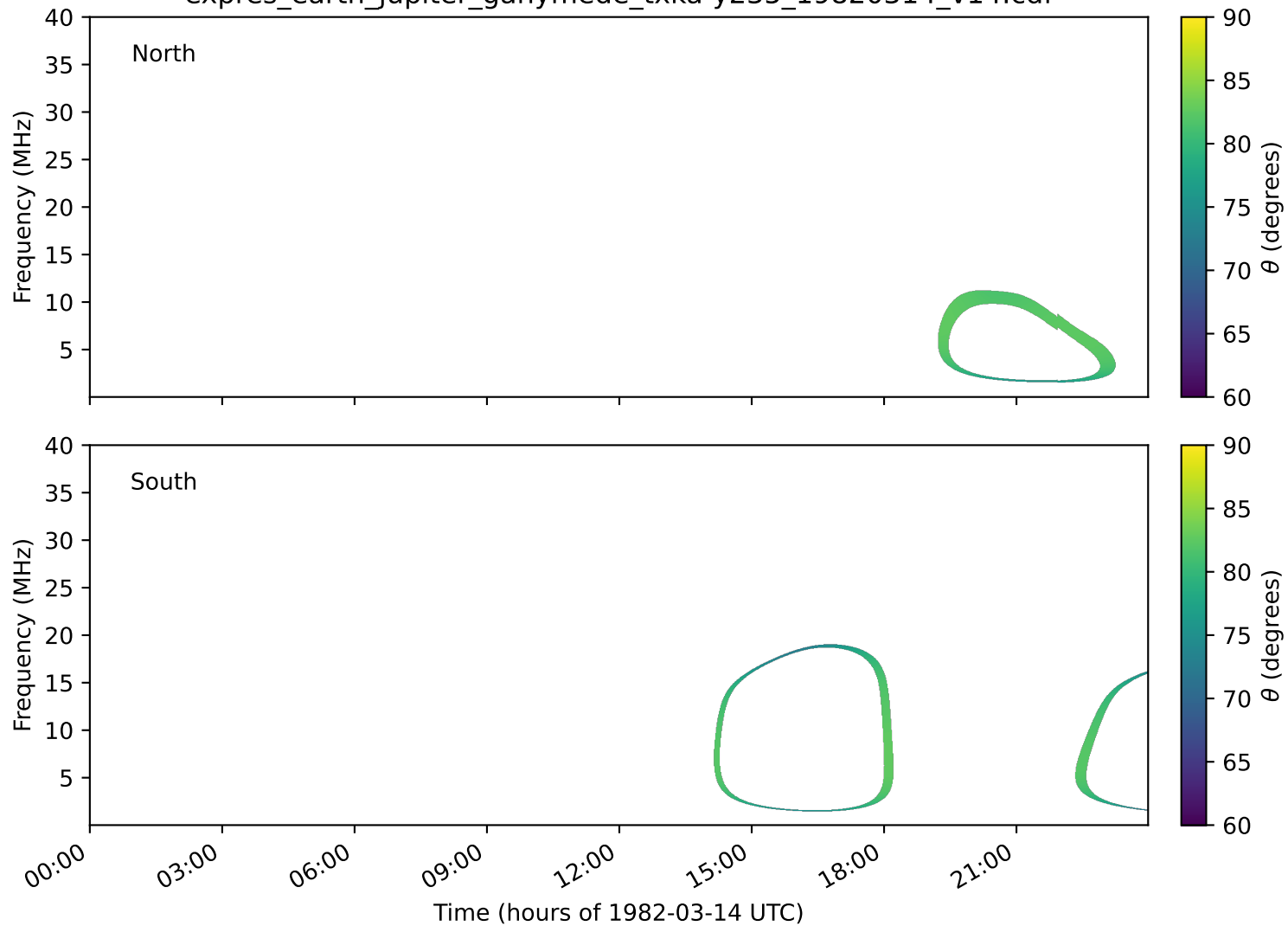
expres_earth_jupiter_ganymede_txka-y235_19820314_v14.cdf
