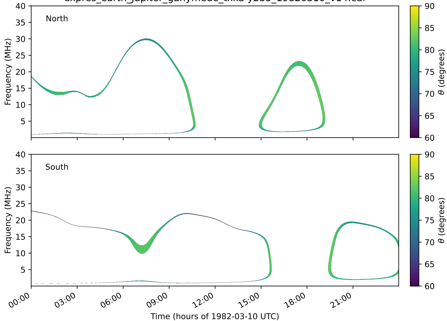
expres_earth_jupiter_ganymede_txka-y235_19820310_v14.cdf
