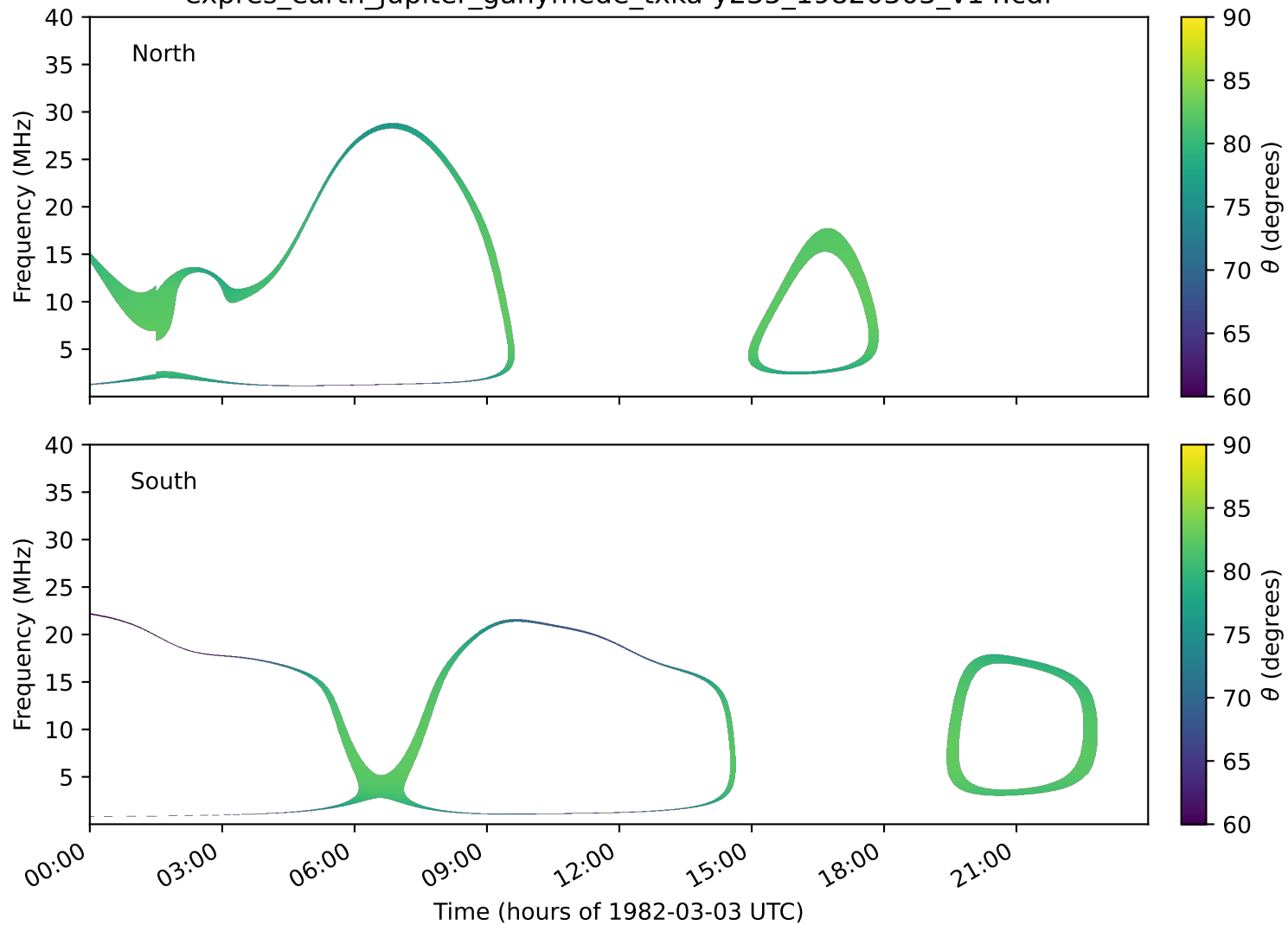
expres_earth_jupiter_ganymede_txka-y235_19820303_v14.cdf
