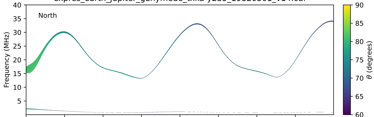
expres_earth_jupiter_ganymede_txka-y235_19820301_v14.cdf
