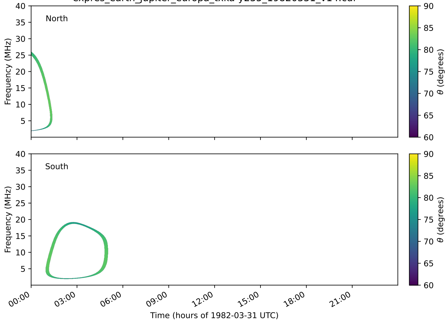
expres_earth_jupiter_europa_txka-y235_19820331_v14.cdf
