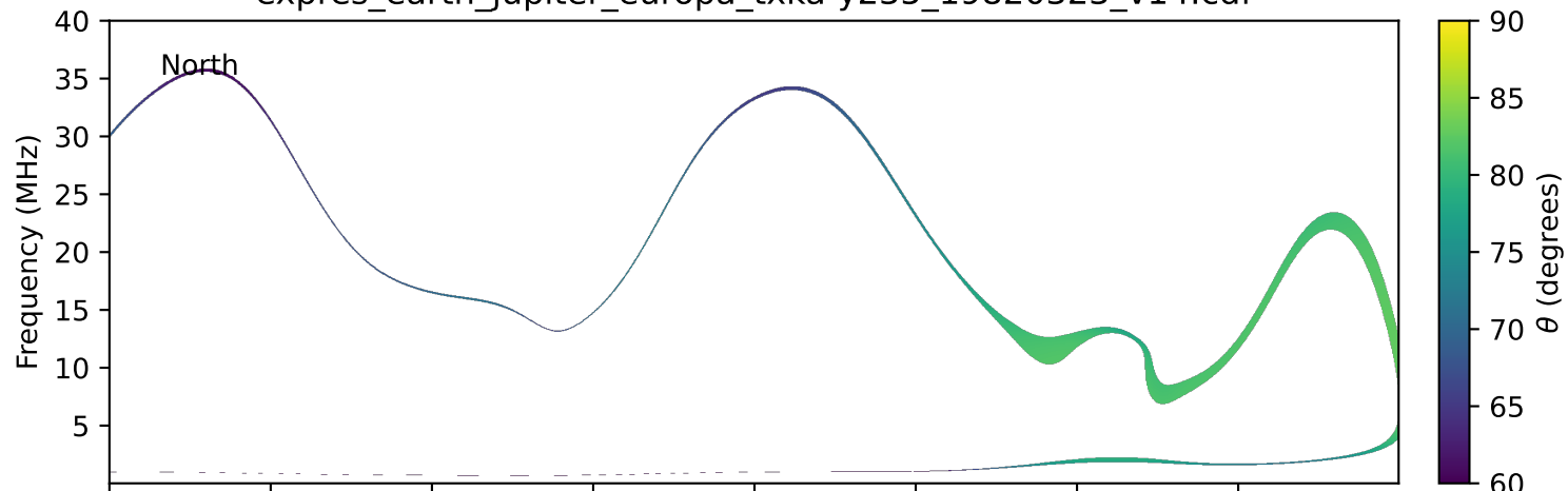
expres_earth_jupiter_europa_txka-y235_19820323_v14.cdf
