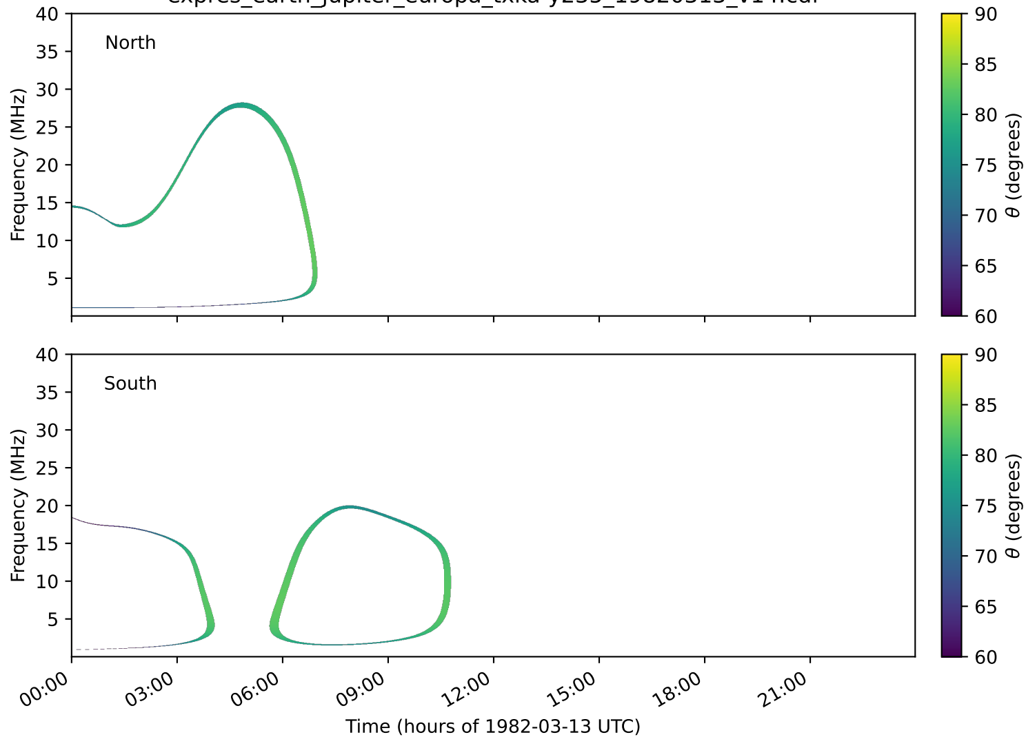
expres_earth_jupiter_europa_txka-y235_19820313_v14.cdf
