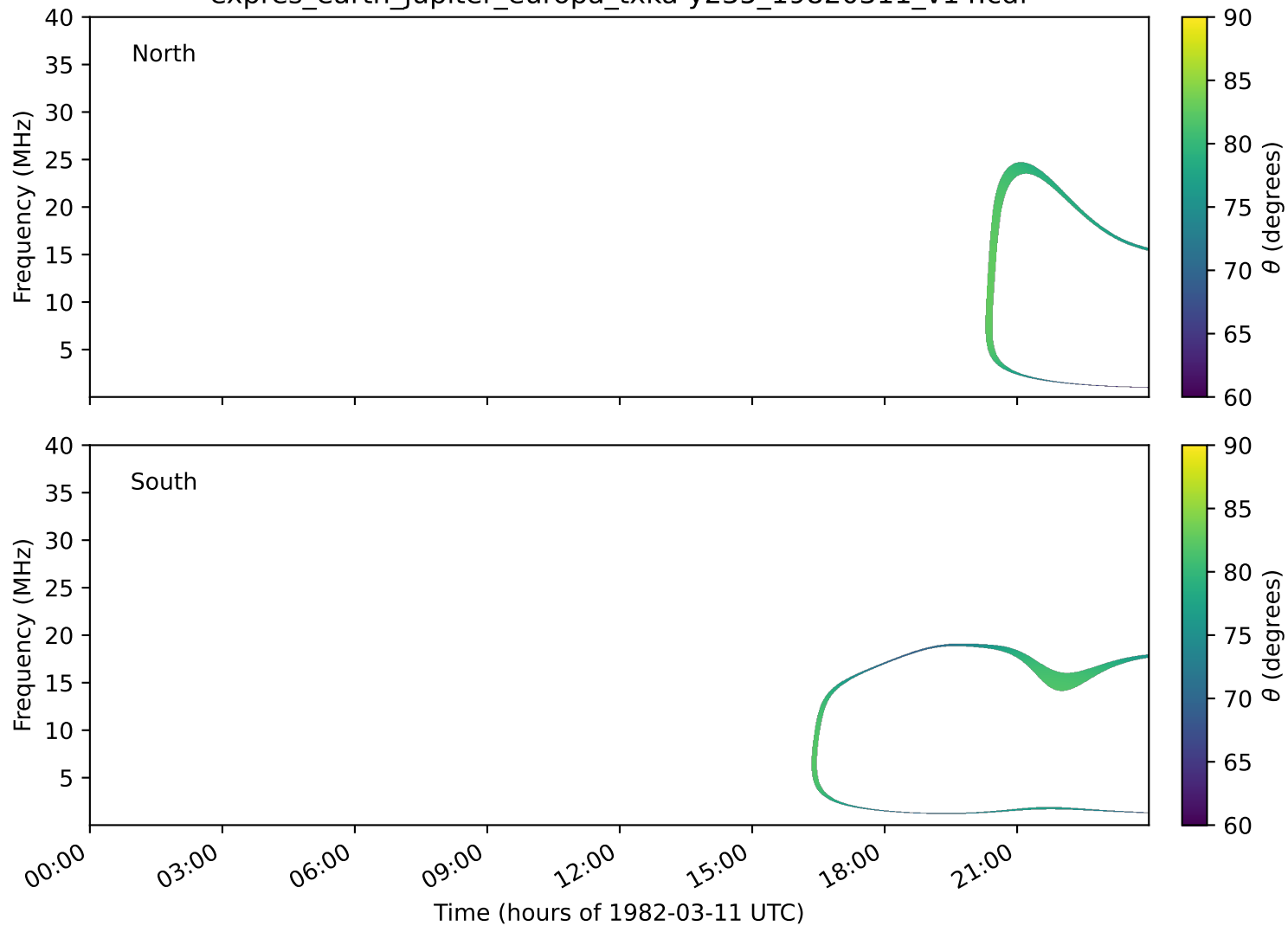
expres_earth_jupiter_europa_txka-y235_19820311_v14.cdf
