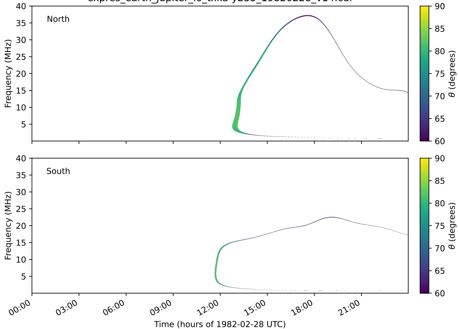
expres_earth_jupiter_io_txka-y235_19820228_v14.cdf
