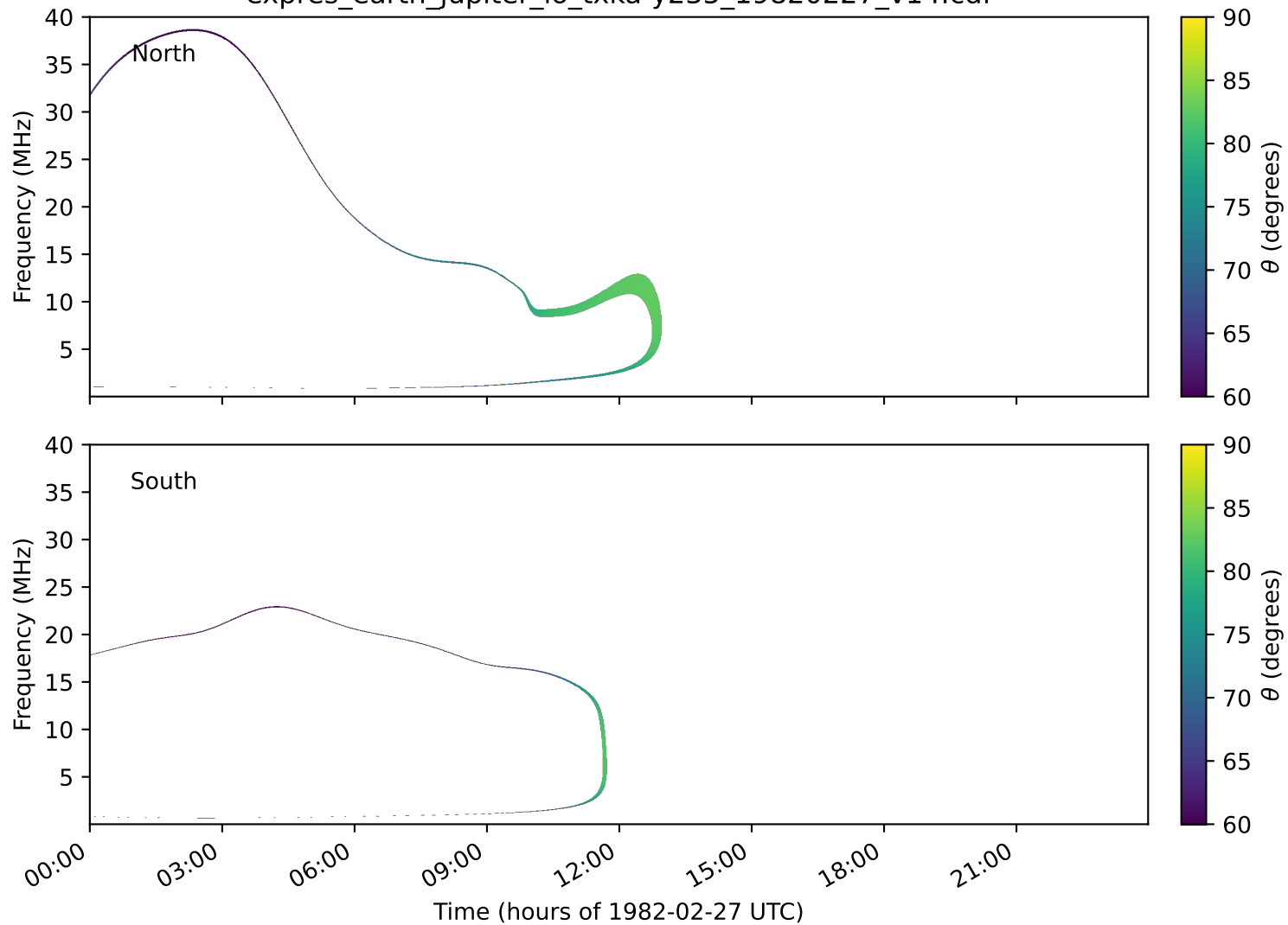
expres_earth_jupiter_io_txka-y235_19820227_v14.cdf
