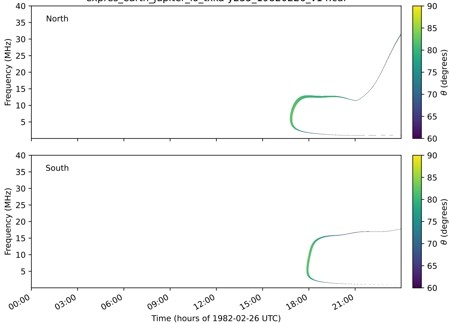
expres_earth_jupiter_io_txka-y235_19820226_v14.cdf
