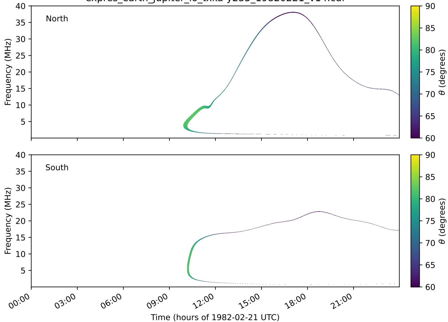
expres_earth_jupiter_io_txka-y235_19820221_v14.cdf
