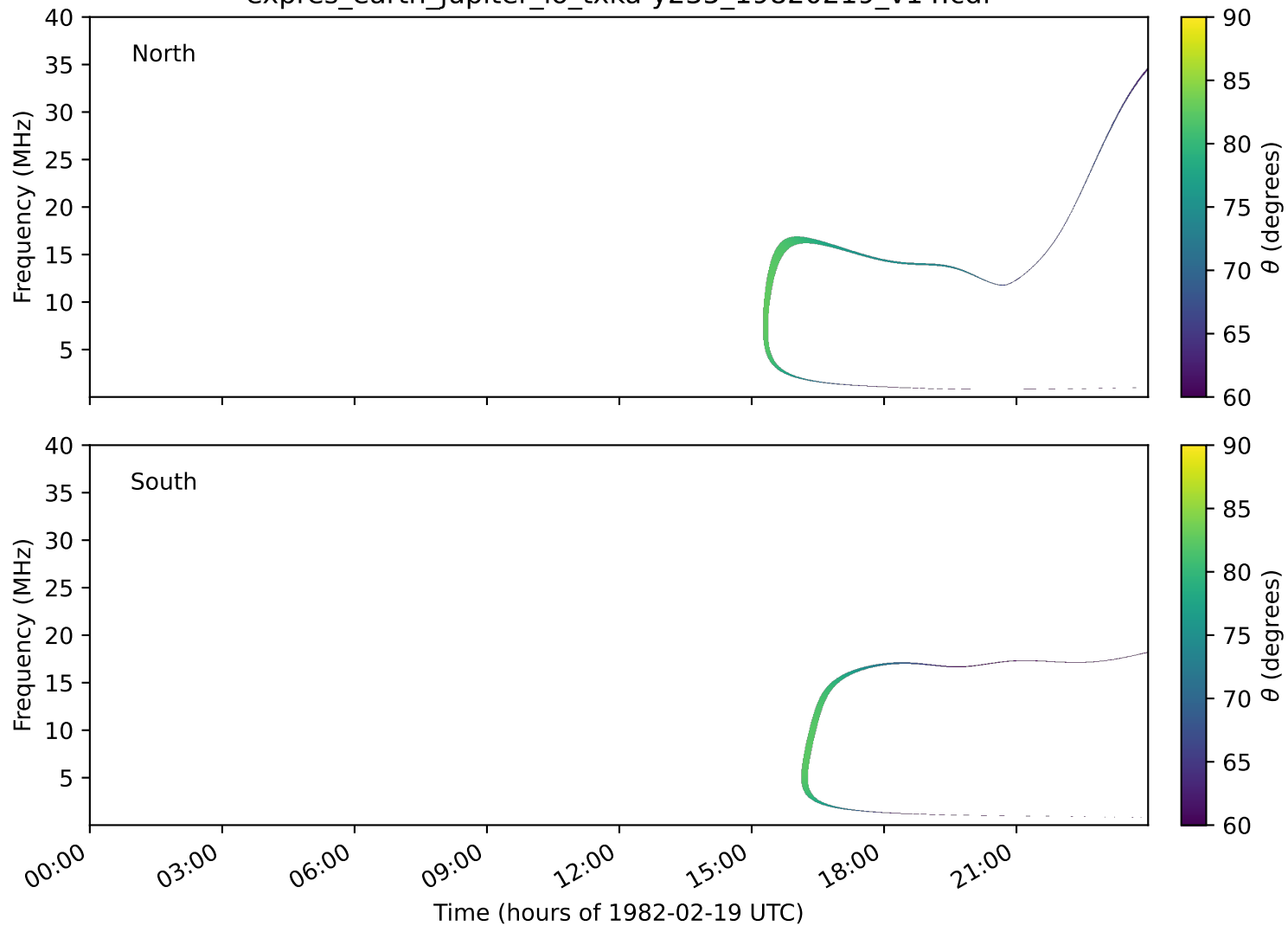
expres_earth_jupiter_io_txka-y235_19820219_v14.cdf
