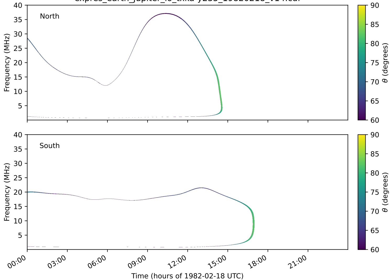
expres_earth_jupiter_io_txka-y235_19820218_v14.cdf
