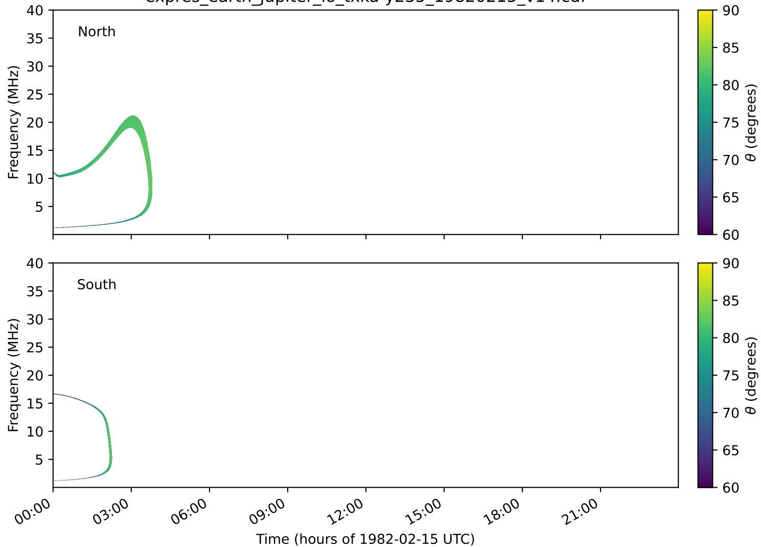
expres_earth_jupiter_io_txka-y235_19820215_v14.cdf
