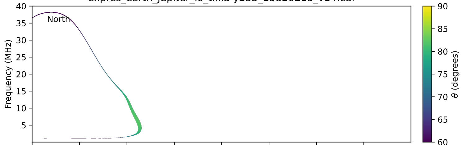
expres_earth_jupiter_io_txka-y235_19820213_v14.cdf
