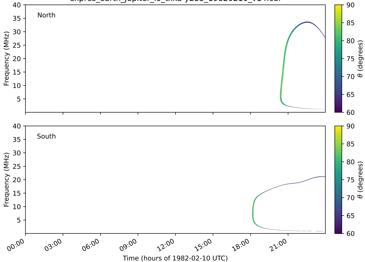
expres_earth_jupiter_io_txka-y235_19820210_v14.cdf
