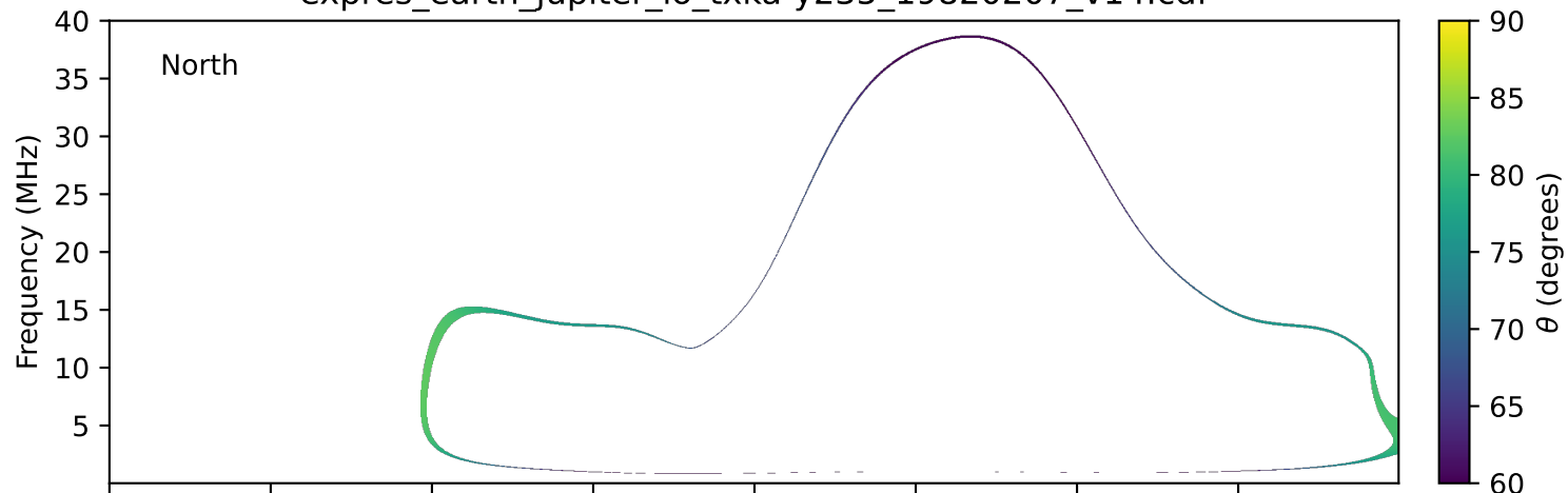
expres_earth_jupiter_io_txka-y235_19820207_v14.cdf
