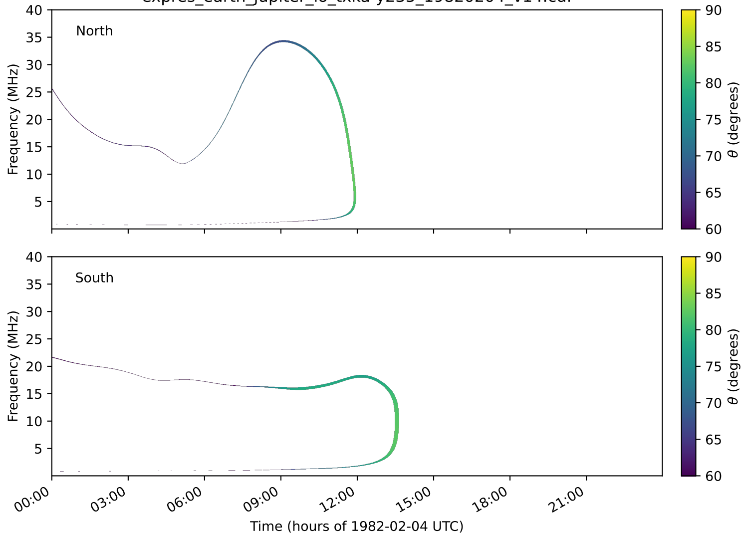
expres_earth_jupiter_io_txka-y235_19820204_v14.cdf
