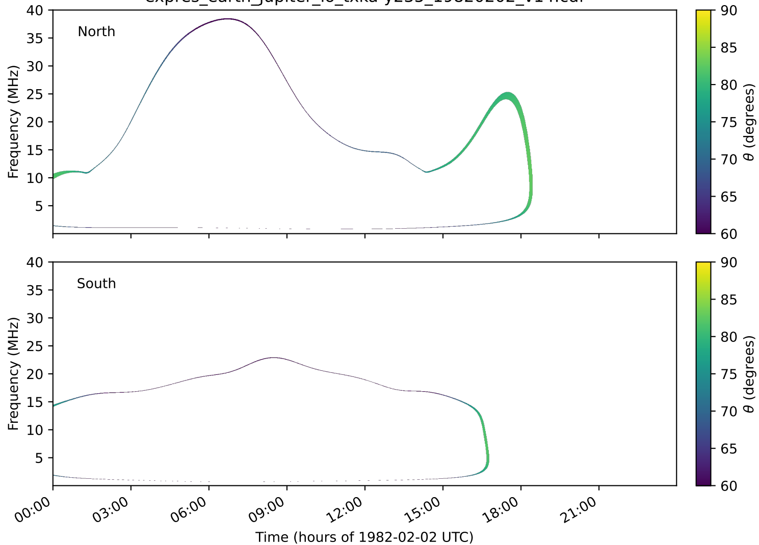
expres_earth_jupiter_io_txka-y235_19820202_v14.cdf
