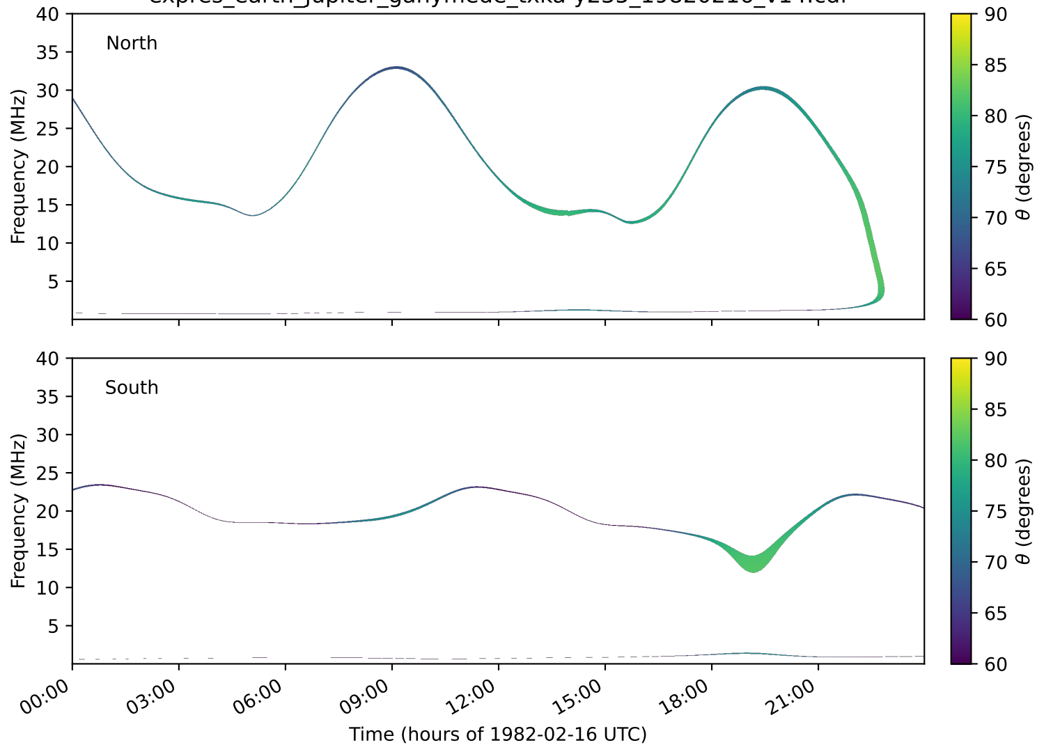
expres_earth_jupiter_ganymede_txka-y235_19820216_v14.cdf
