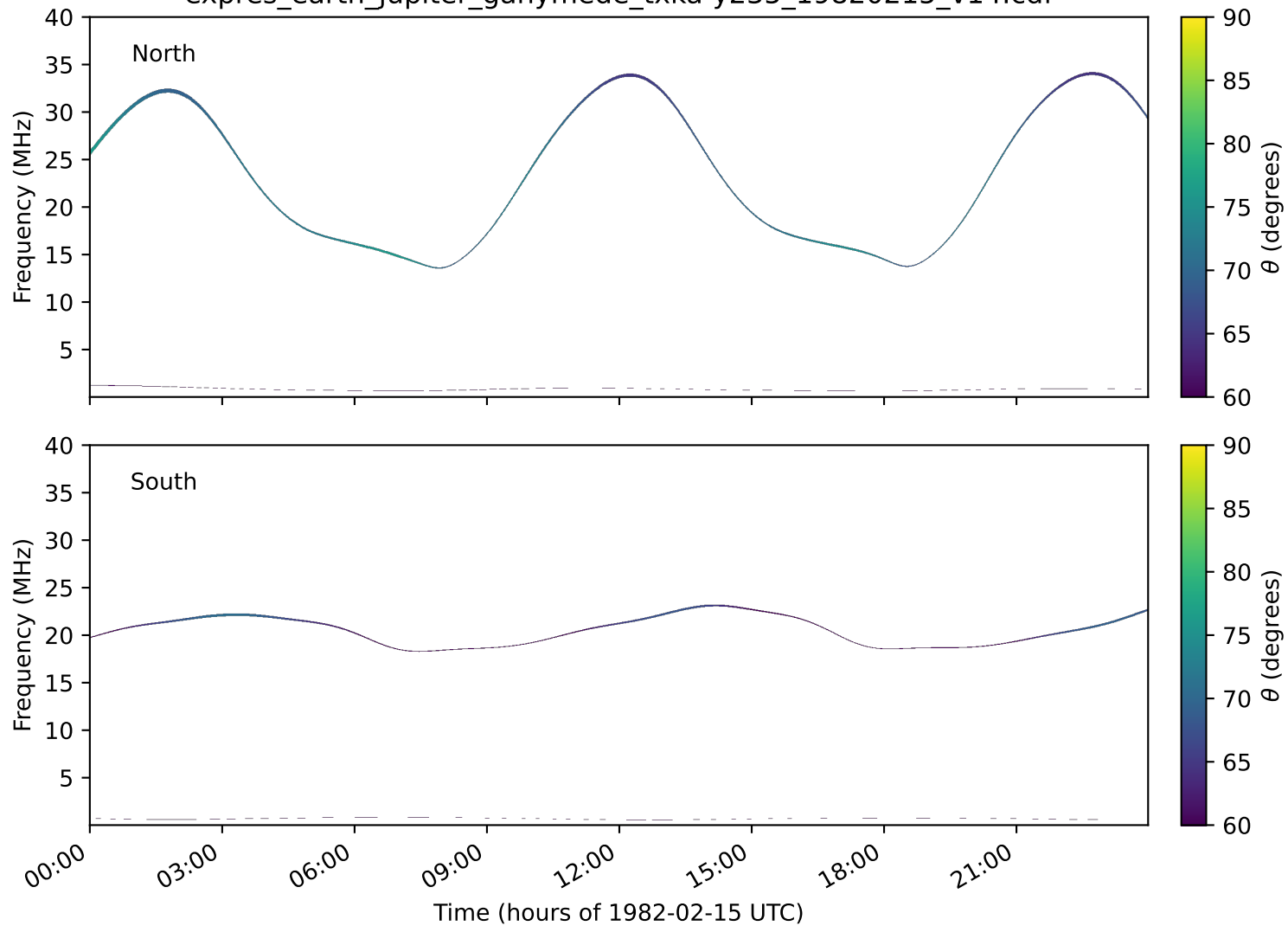
expres_earth_jupiter_ganymede_txka-y235_19820215_v14.cdf
