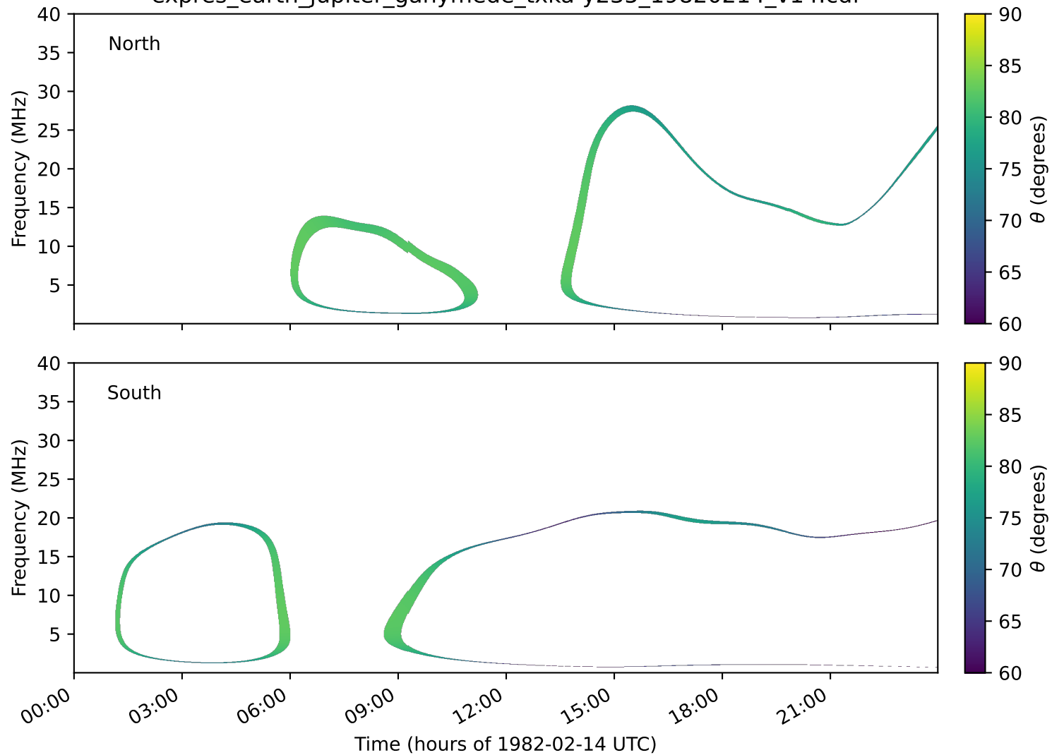
expres_earth_jupiter_ganymede_txka-y235_19820214_v14.cdf
