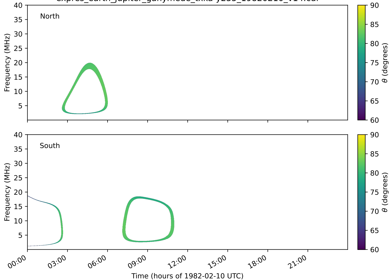
expres_earth_jupiter_ganymede_txka-y235_19820210_v14.cdf
