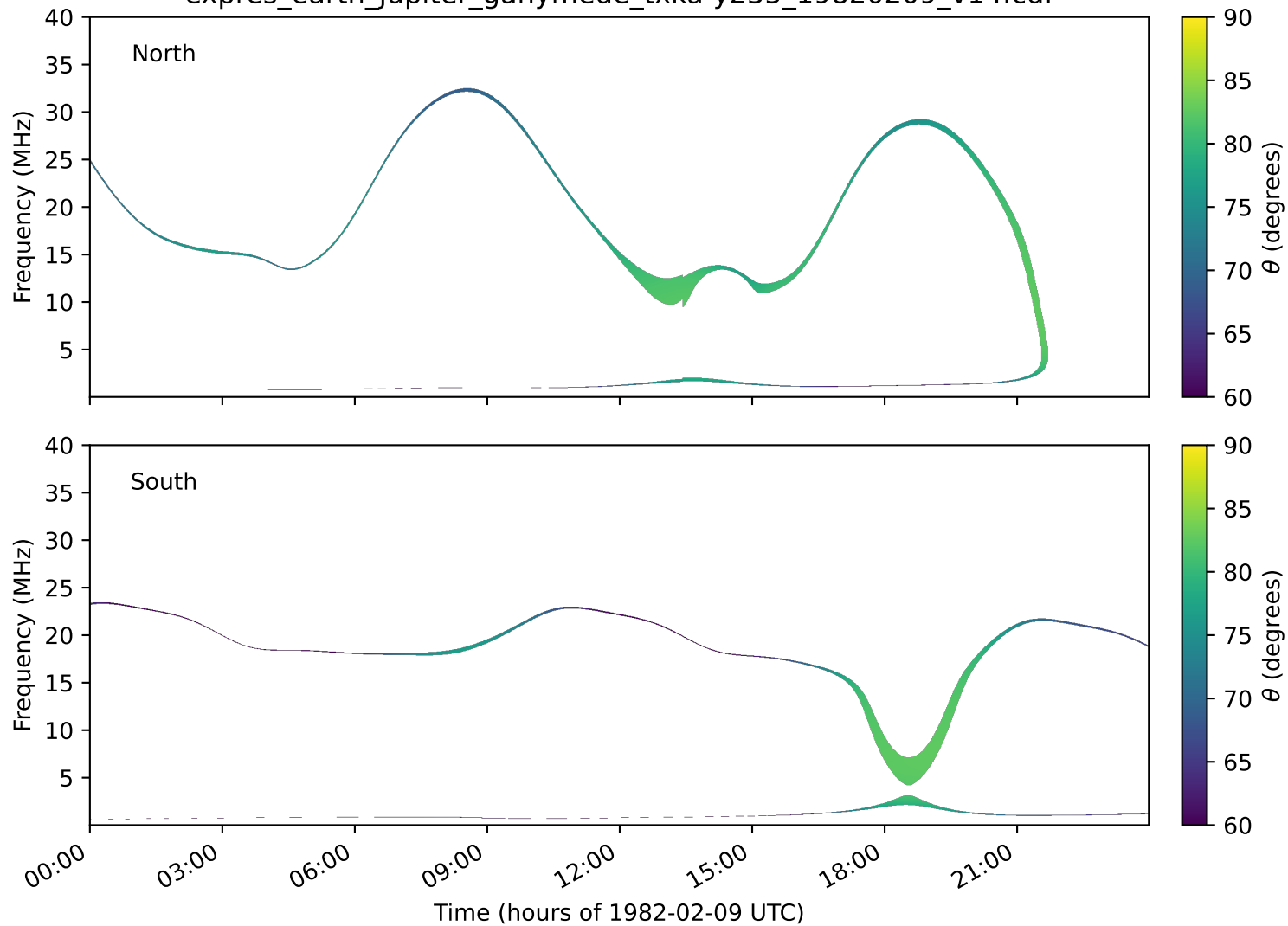
expres_earth_jupiter_ganymede_txka-y235_19820209_v14.cdf
