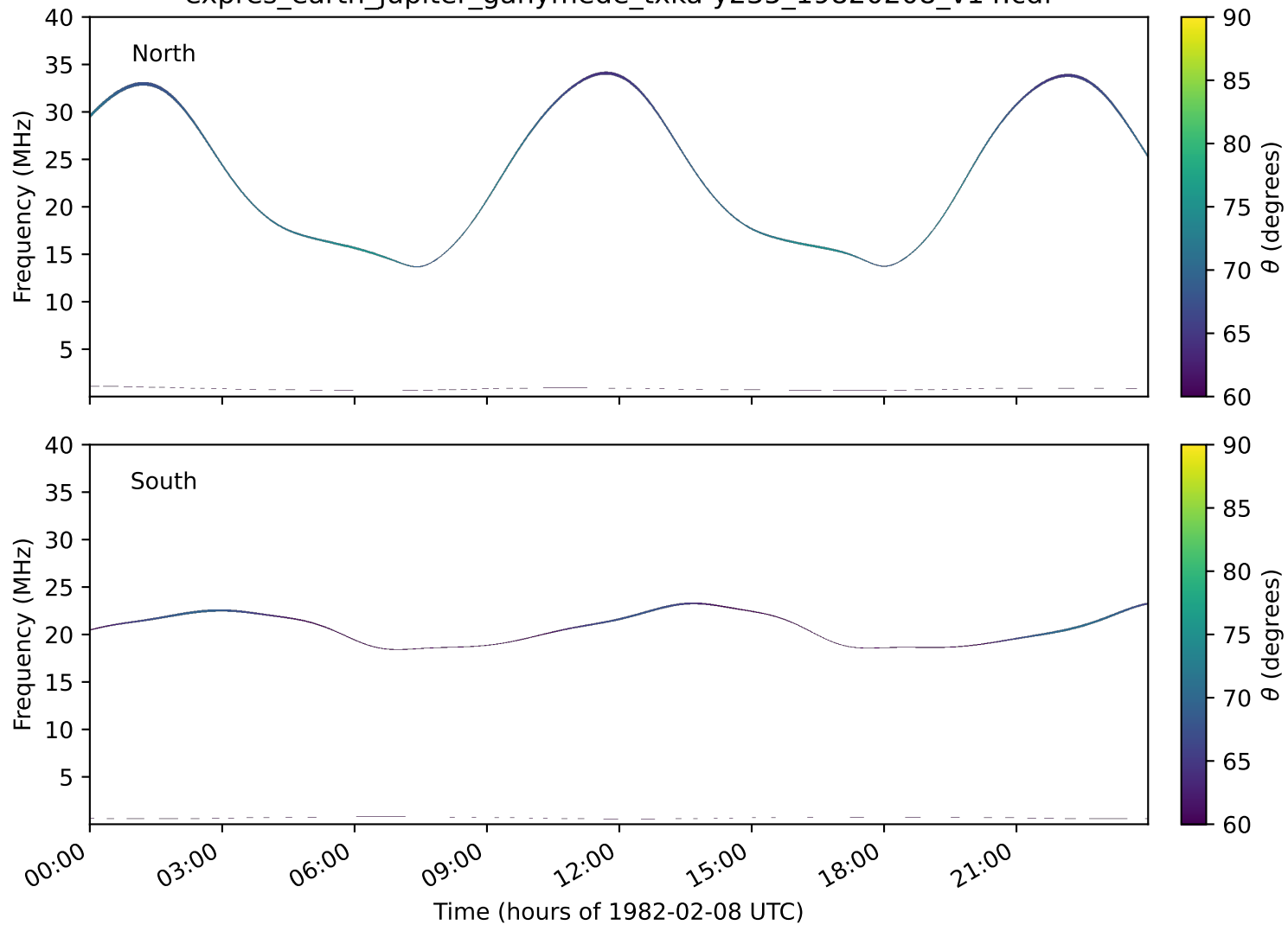
expres_earth_jupiter_ganymede_txka-y235_19820208_v14.cdf
