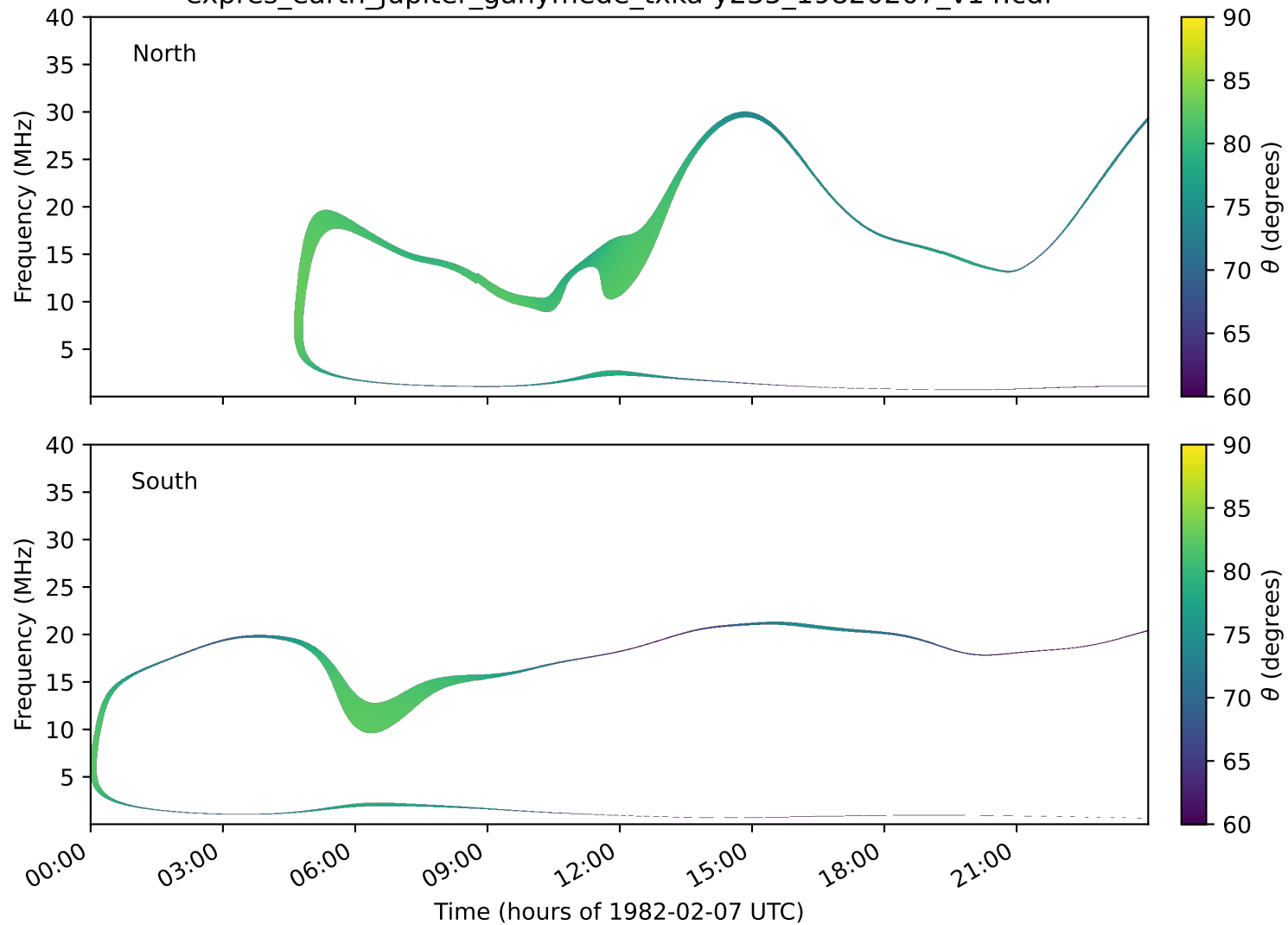
expres_earth_jupiter_ganymede_txka-y235_19820207_v14.cdf
