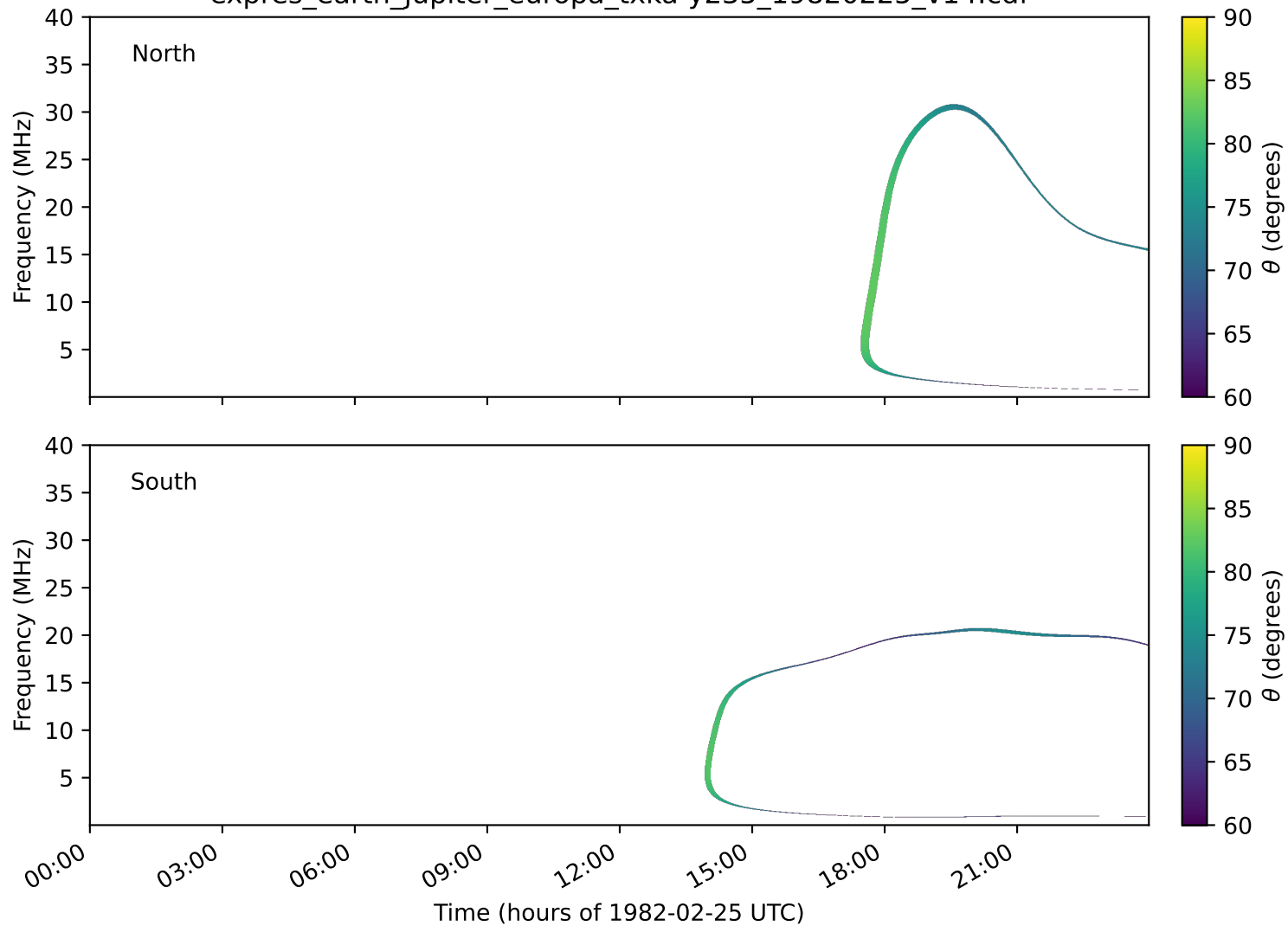
expres_earth_jupiter_europa_txka-y235_19820225_v14.cdf
