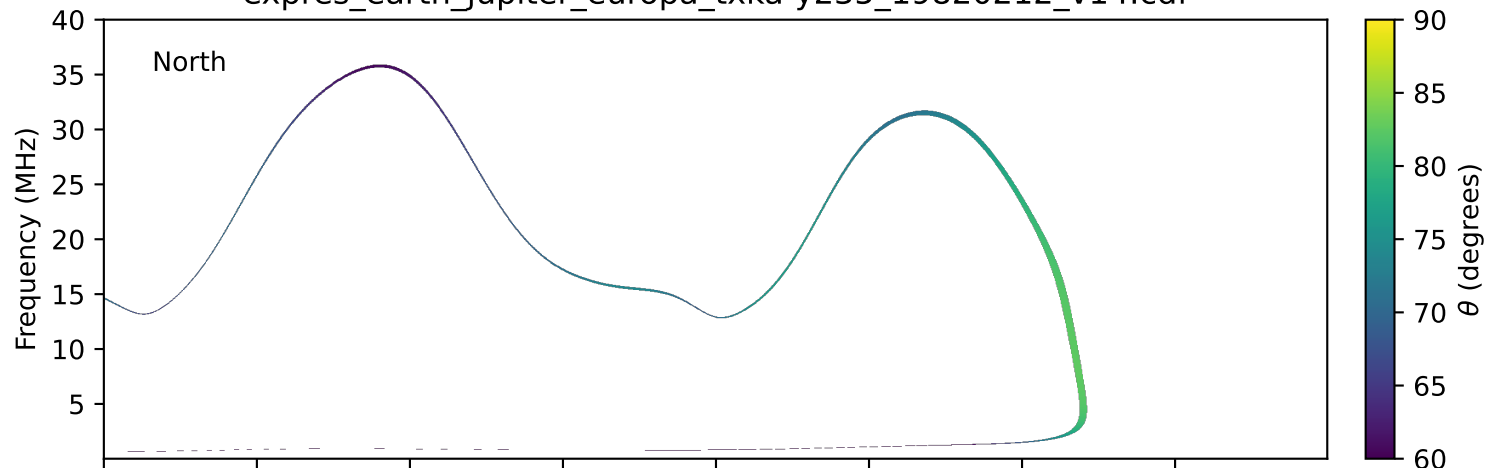
expres_earth_jupiter_europa_txka-y235_19820212_v14.cdf
