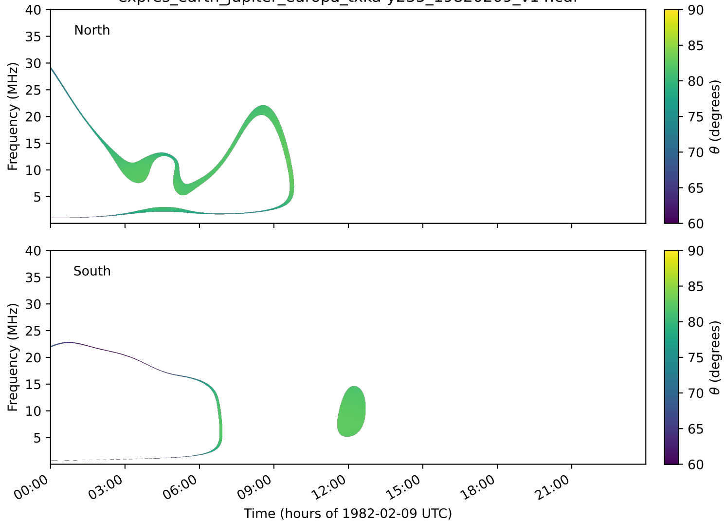
expres_earth_jupiter_europa_txka-y235_19820209_v14.cdf
