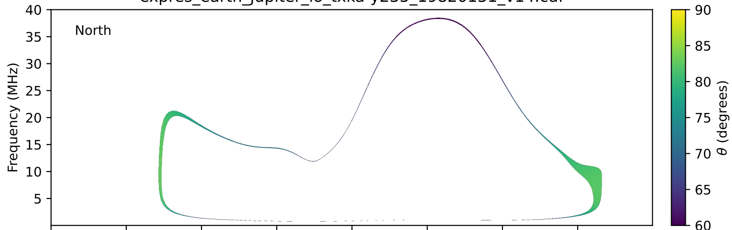
expres_earth_jupiter_io_txka-y235_19820131_v14.cdf
