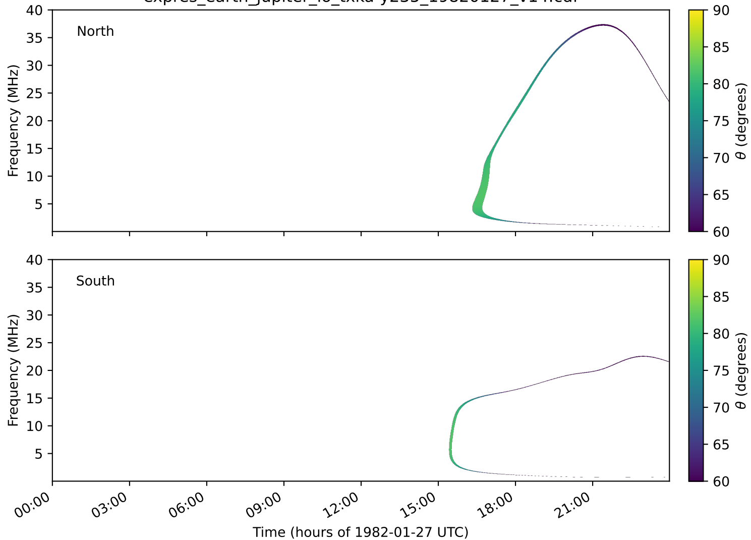
expres_earth_jupiter_io_txka-y235_19820127_v14.cdf
