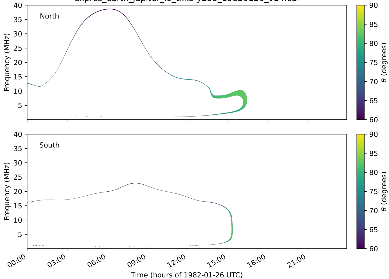
expres_earth_jupiter_io_txka-y235_19820126_v14.cdf
