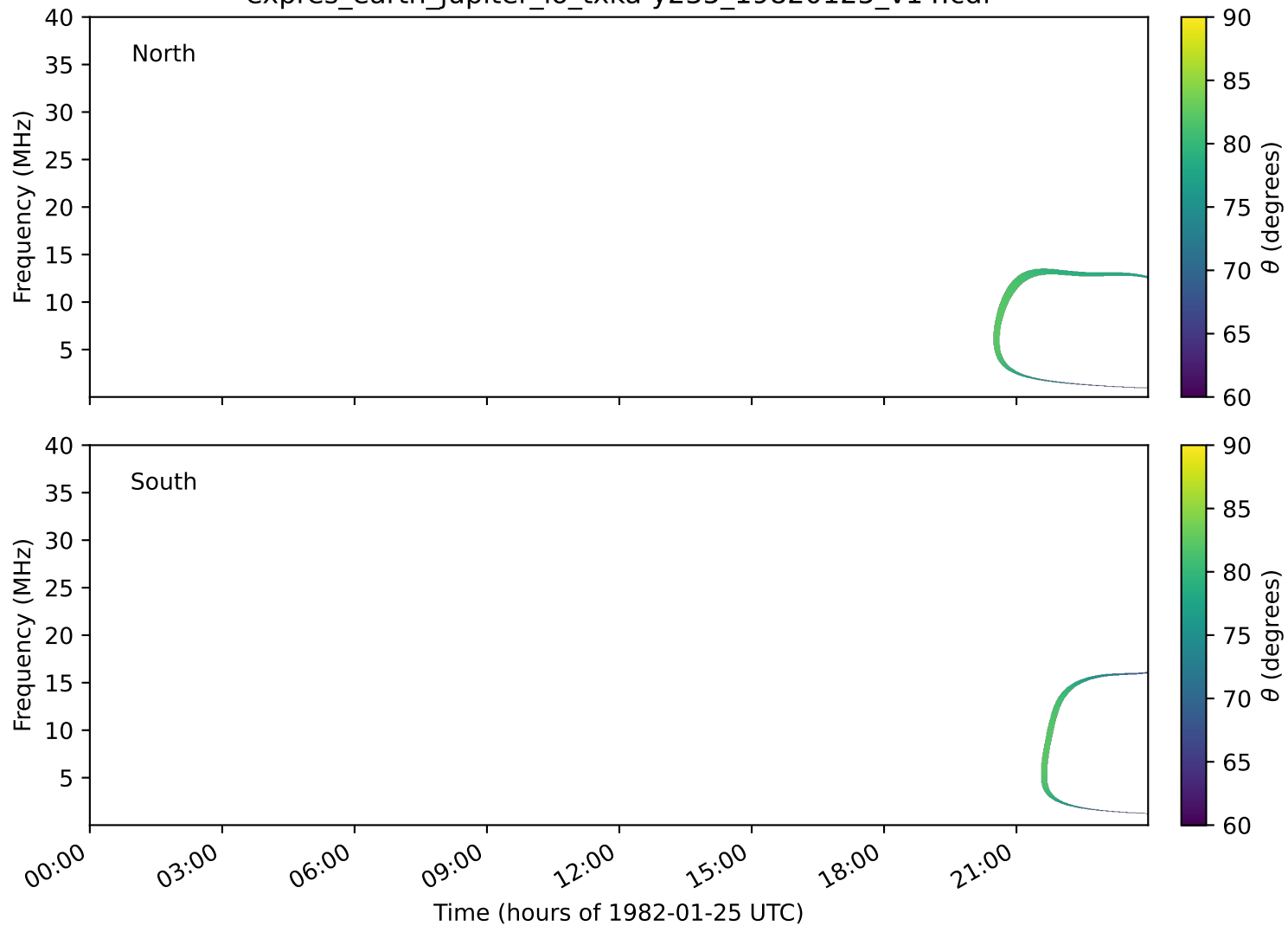
expres_earth_jupiter_io_txka-y235_19820125_v14.cdf
