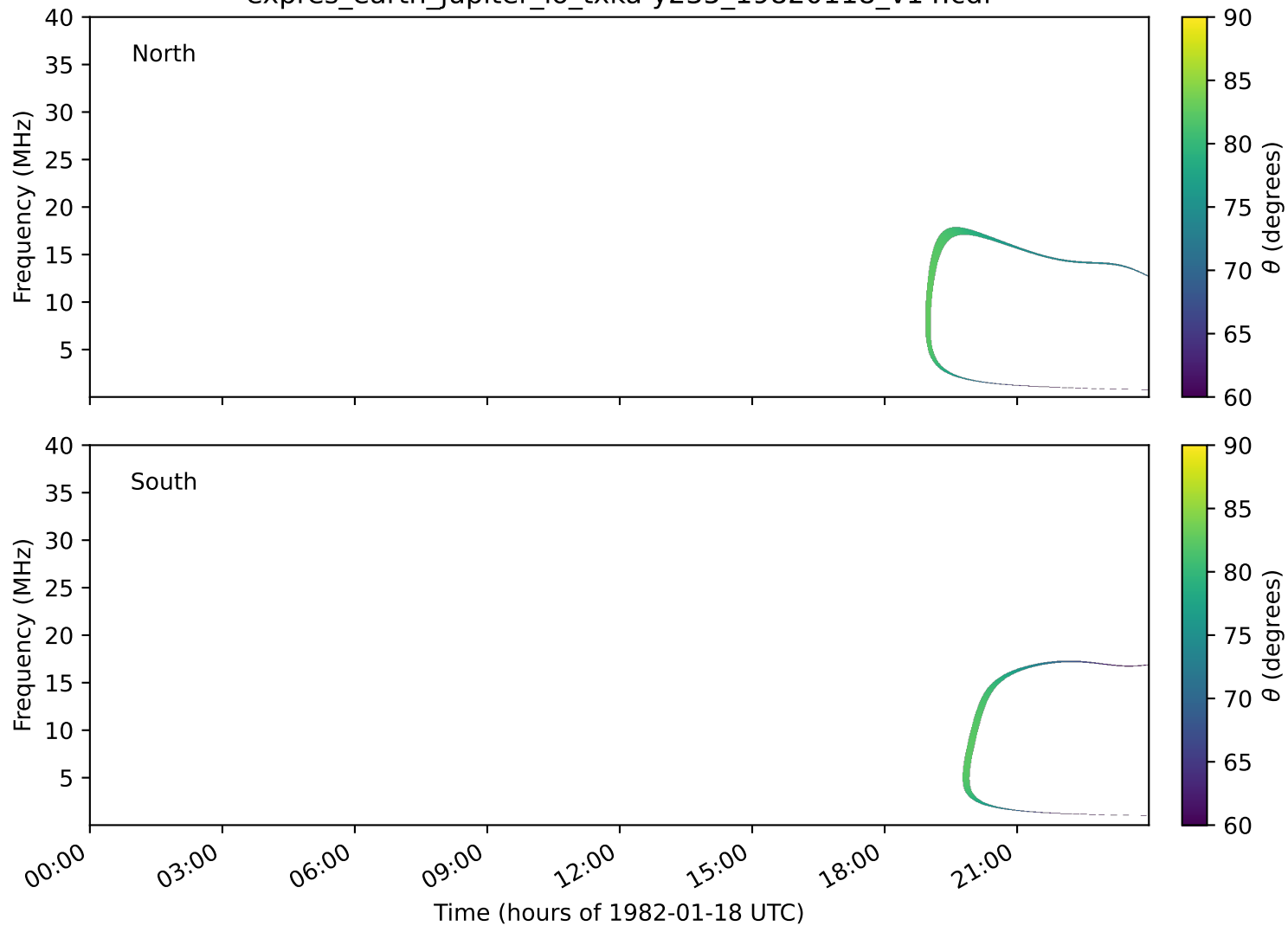
expres_earth_jupiter_io_txka-y235_19820118_v14.cdf
