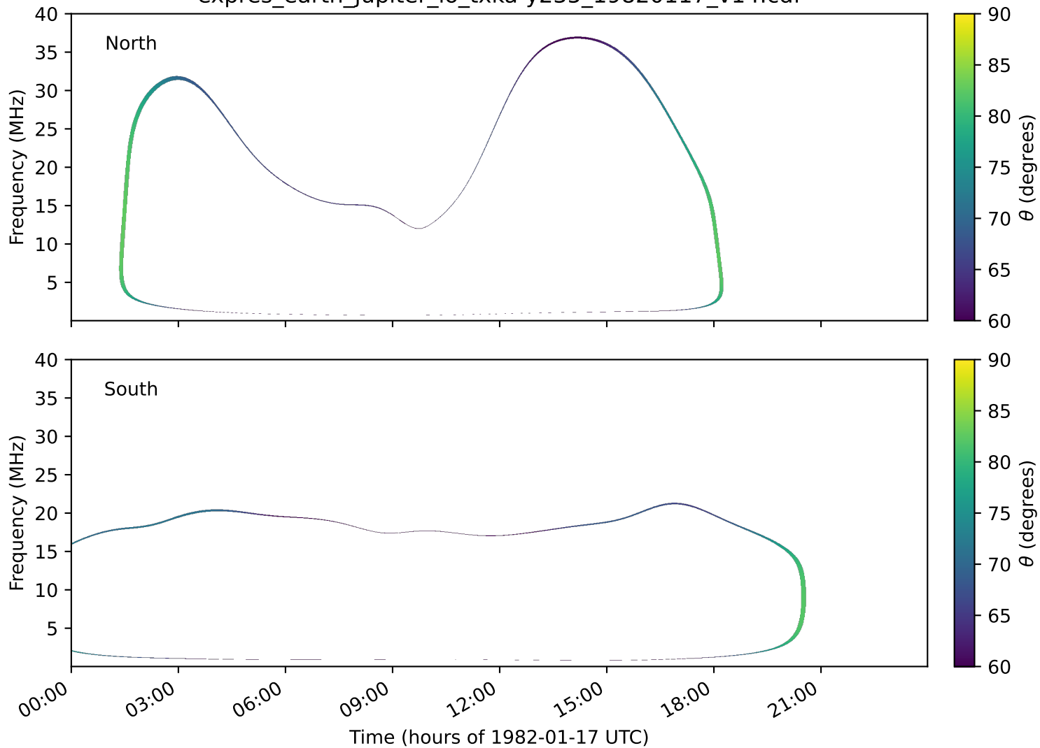
expres_earth_jupiter_io_txka-y235_19820117_v14.cdf
