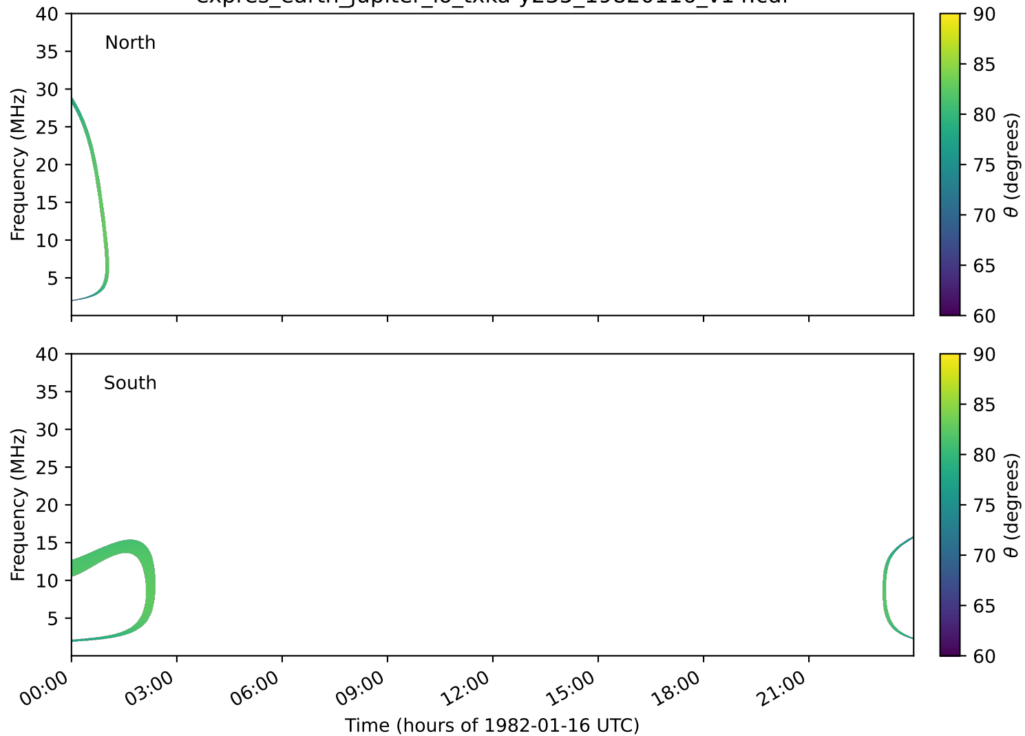
expres_earth_jupiter_io_txka-y235_19820116_v14.cdf
