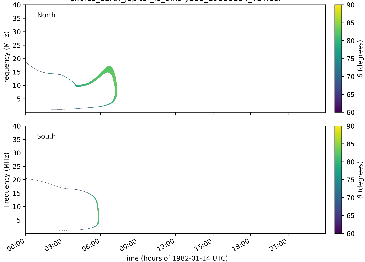
expres_earth_jupiter_io_txka-y235_19820114_v14.cdf
