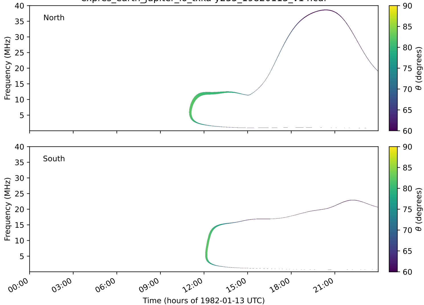
expres_earth_jupiter_io_txka-y235_19820113_v14.cdf
