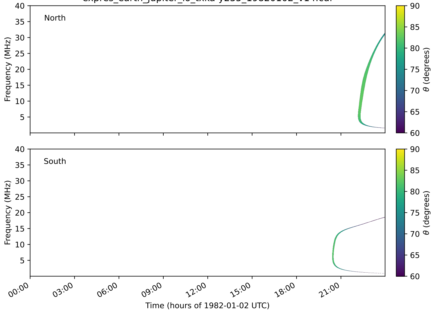
expres_earth_jupiter_io_txka-y235_19820102_v14.cdf
