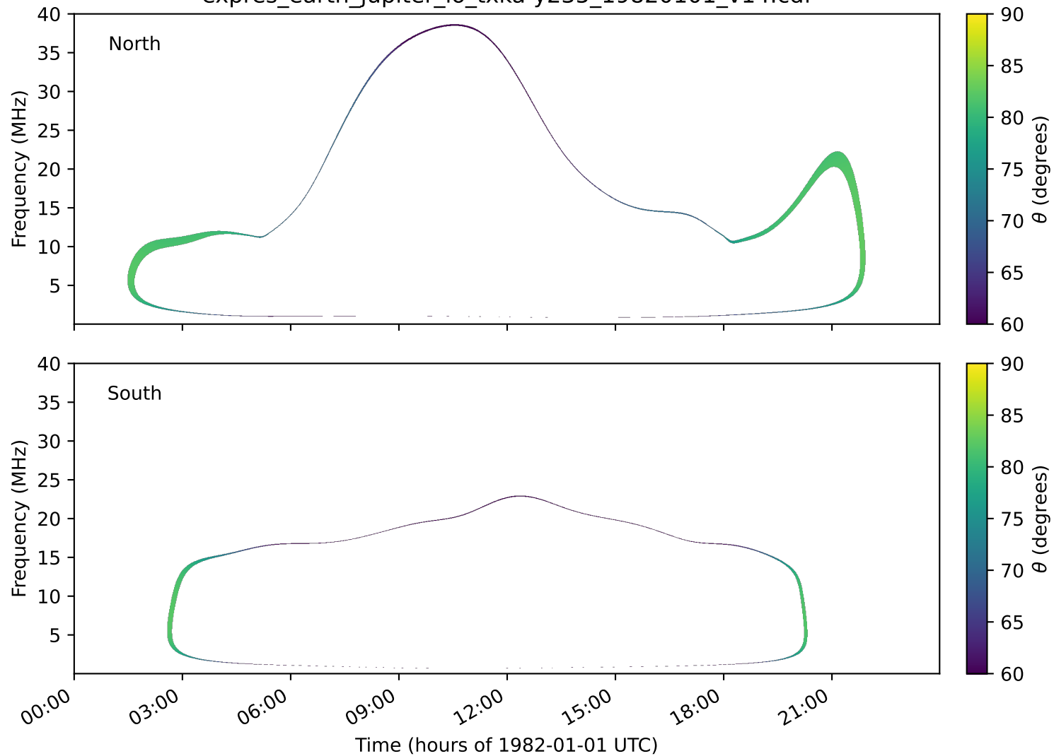
expres_earth_jupiter_io_txka-y235_19820101_v14.cdf
