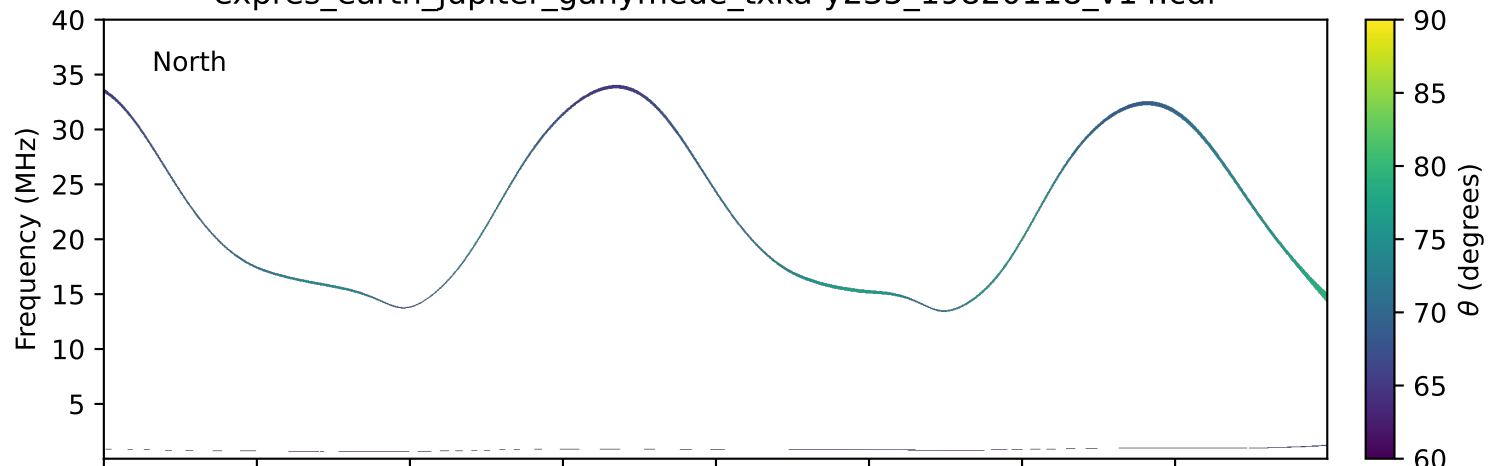
expres_earth_jupiter_ganymede_txka-y235_19820118_v14.cdf
