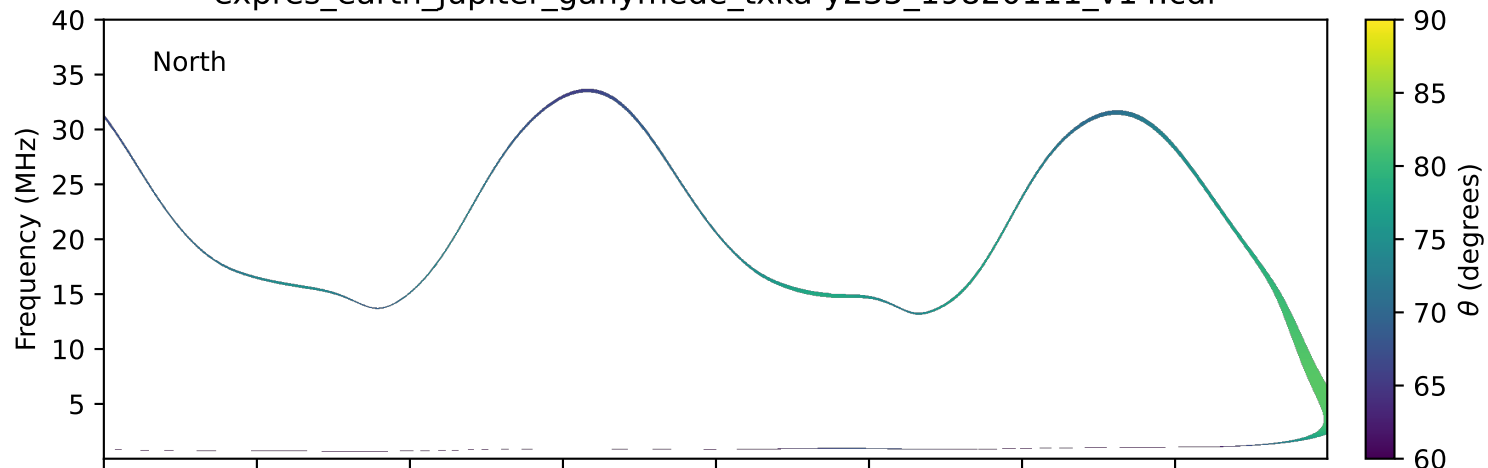
expres_earth_jupiter_ganymede_txka-y235_19820111_v14.cdf
