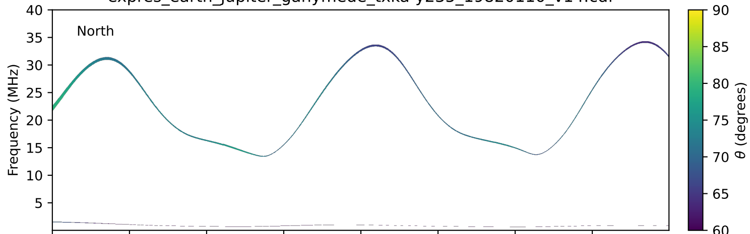
expres_earth_jupiter_ganymede_txka-y235_19820110_v14.cdf
