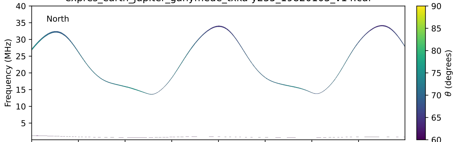
expres_earth_jupiter_ganymede_txka-y235_19820103_v14.cdf
