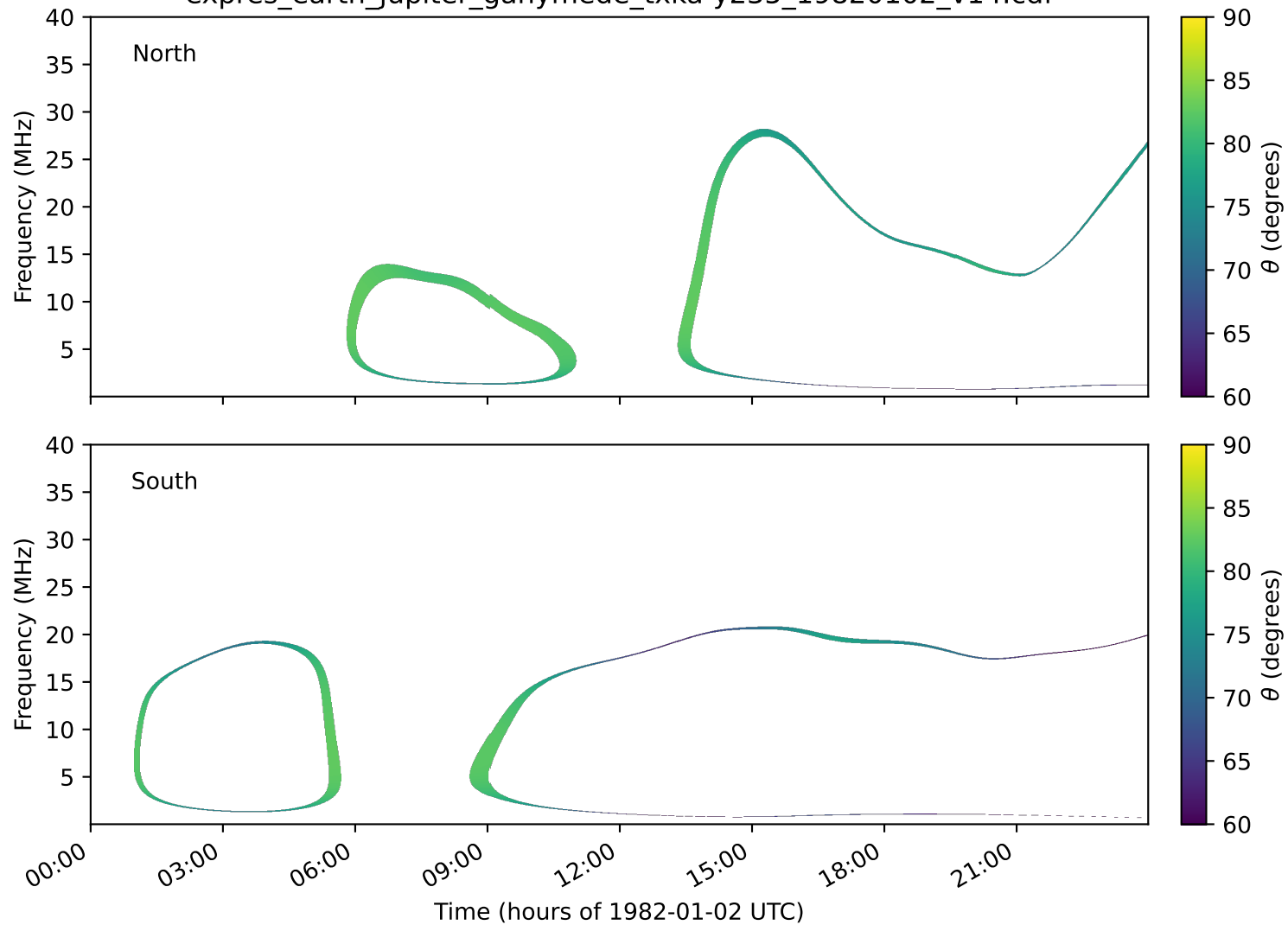
expres_earth_jupiter_ganymede_txka-y235_19820102_v14.cdf
